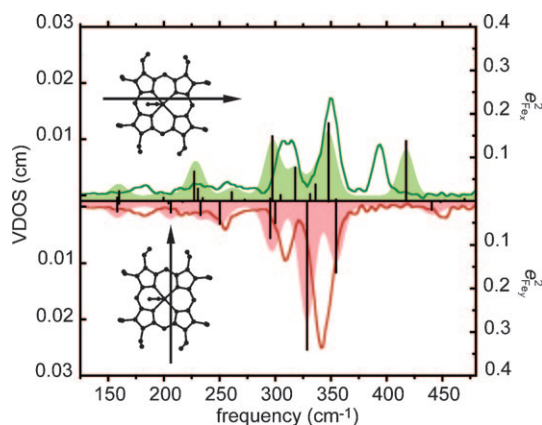
Figure 3. Measured (lines) and predicted (shaded) contributions to the VDOS from Fe atom motion along x (green) and y (red) directions, together with calculated e_{\text{Fe}x}^2 , e_{\text{Fe}y}^2 values (bars) over the 125–480 \text{cm}^{-1} region. Porphyrin diagrams to the left present the in-plane directions of Fe motion, parallel (top panel) and perpendicular to the FeNO plane (bottom panel).
