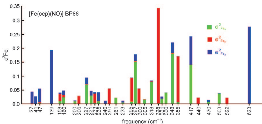
Figure 5. Bar graph showing DFT-predicted directional characteristics of all 32 modes with e_{\text{Fe}x}^2 > 0.01 . NRVS x green; NRVS y red; NRVS z blue. The values of the predicted frequencies are given at each tick mark, but the horizontal scale is only approximately linear in frequency to avoid overlaps.
